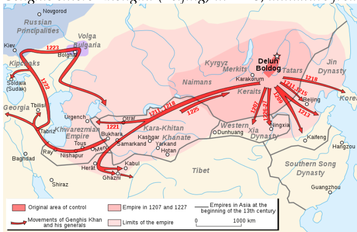
The campaigns Genghis Khan in the period 1207-1225
